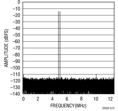
LTC2203: 32K Point 2-Tone FFT, f IN = 4.9MHz and 30.1MHz, -15dBFS, PGA = 0
