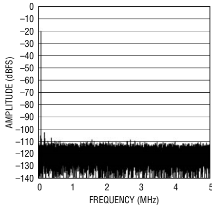
LTC2202: 32K Point FFT, f IN = 70.1MHz, -20dBFS, PGA = 1
