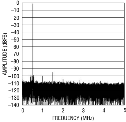
LTC2202: 32K Point FFT, f IN = 30.5MHz, -1dBFS, PGA = 1
