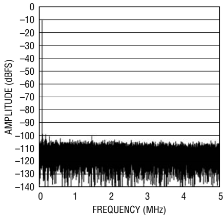
LTC2202: 32K Point FFT, f IN = 70.1MHz, -10dBFS, PGA = 1
