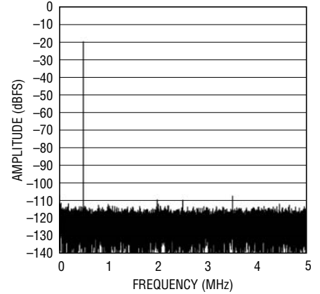
LTC2202: 32K Point FFT, f IN = 30.5MHz, -20dBFS, PGA = 1
