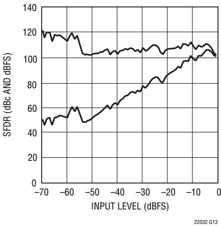
LTC2203: SFDR vs Input Level, f IN = 5MHz, PGA = 0, Dither "Off"
