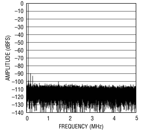
LTC2202: 32K Point FFT, f IN = 70.1MHz, -1dBFS, PGA = 1
