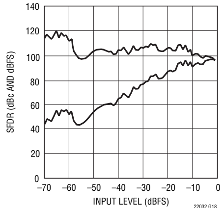
LTC2203: SFDR vs Input Level, f IN = 12.7MHz, PGA = 0, Dither "Off"
