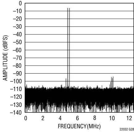
LTC2203: 32K Point 2-Tone FFT, f_{IN} = 44.9\text{MHz} and 70.1\text{MHz} , -7dBFS, PGA = 0
