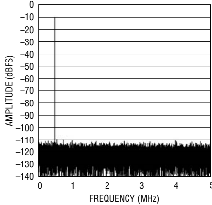
LTC2202: 32K Point FFT, f IN = 30.5MHz, -10dBFS, PGA = 1
