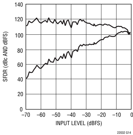
LTC2203: SFDR vs Input Level, f IN = 5MHz, PGA = 0, Dither "On"
