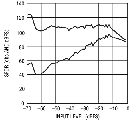
LTC2203: SFDR vs Input Level, f_{IN} = 70.1\text{MHz} , PGA = 0, Dither "Off"
