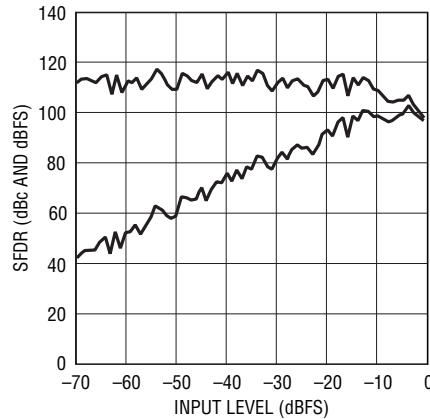
LTC2202: SFDR vs Input Level, f IN = 30.1MHz, PGA = 0, Dither "On"
