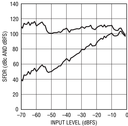
LTC2202: SFDR vs Input Level, f IN = 30.1MHz, PGA = 0, Dither "Off"
