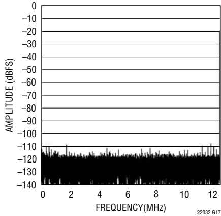
LTC2203: 32K Point FFT, f IN = 12.4MHz, -20dBFS, PGA = 0
