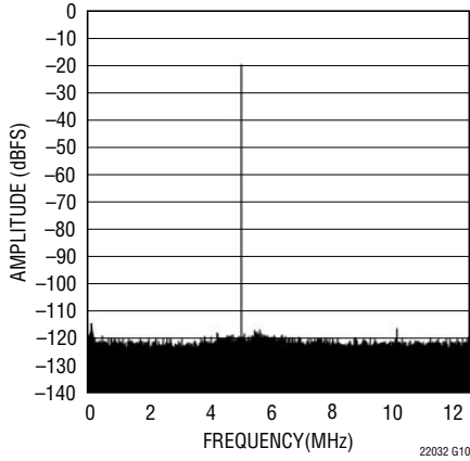
LTC2203: 128K Point FFT, f IN = 5.1MHz, -20dBFS, PGA = 0, Internal Dither "On"
