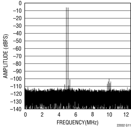
LTC2203: 32K Point 2-Tone FFT, f IN = 4.9MHz and 30.1MHz, -7dBFS, PGA = 0
