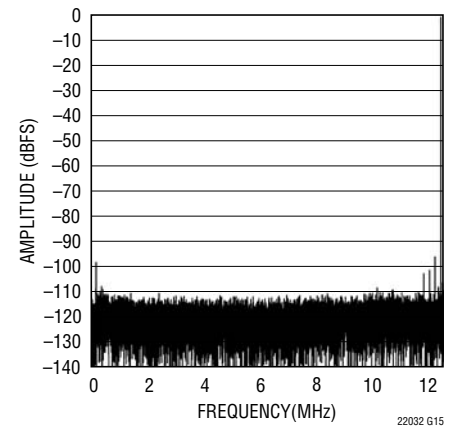
LTC2203: 32K Point FFT, f IN = 12.4MHz, -1dBFS, PGA = 0
