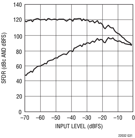
LTC2203: SFDR vs Input Level, f_{IN} = 70.1\text{MHz} , PGA = 0, Dither "On"
