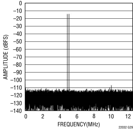
LTC2203: 32K Point 2-Tone FFT, f_{IN} = 44.9\text{MHz} and 70.1\text{MHz} , -15dBFS, PGA = 0
