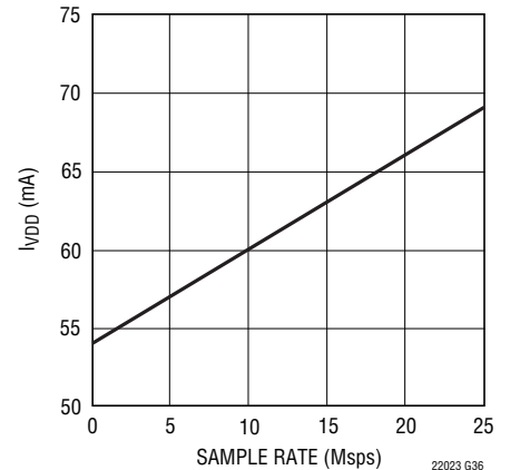
LTC2203: I_{VDD} vs Sample Rate, 5MHz Sine Wave, -1dBFS
